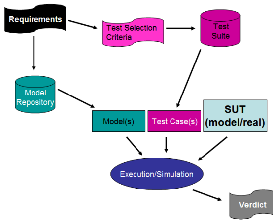
Figure 1: Graphical process extended further from [Utt06]
