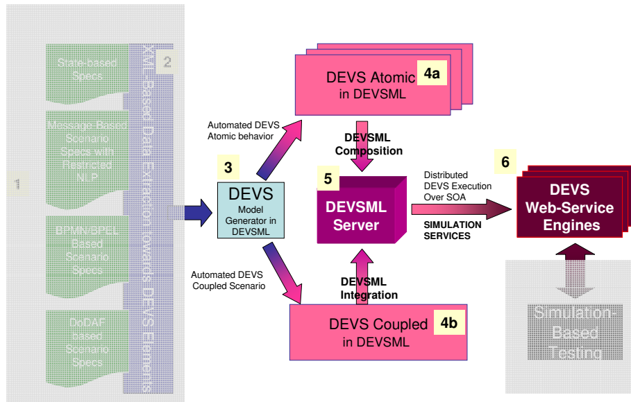
Figure 4: Net-centric collaboration and execution using DEVSSML and DEVSS/SOA
