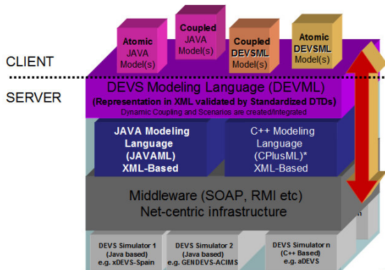
Figure 5: DEVS Transparency and Net-centric model interoperability using DEVSSML. Client and Server categorization is done for DEVSS/SOA implementation
