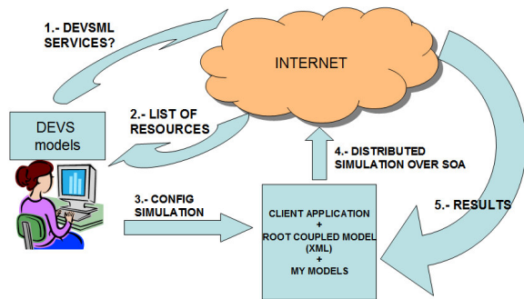
Figure 6: Execution of DEVS SOA-Based M&S
